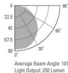
Indoor Distribution Curve (GX-5)
